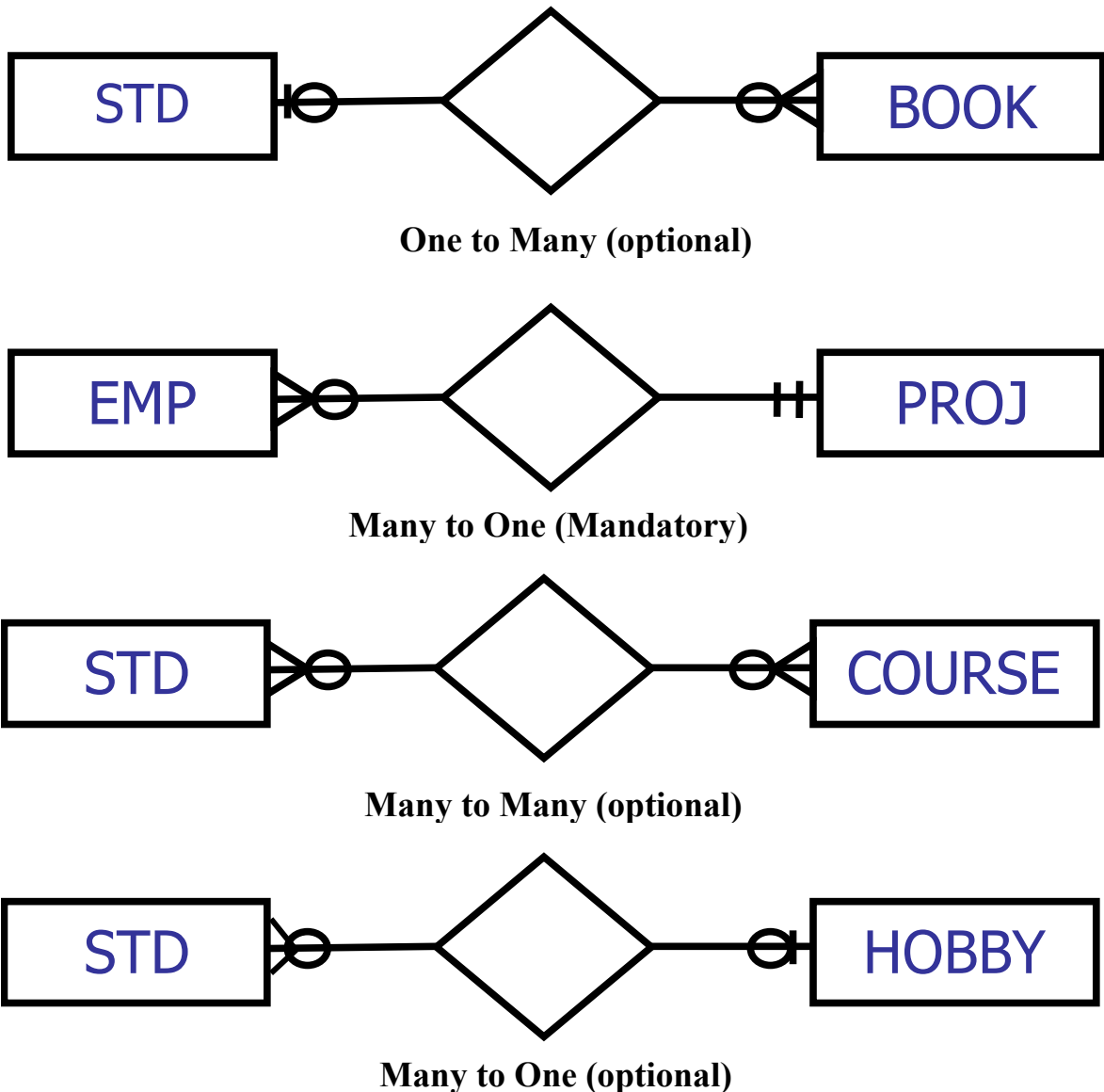
Fig 1: Different Cardinalities
