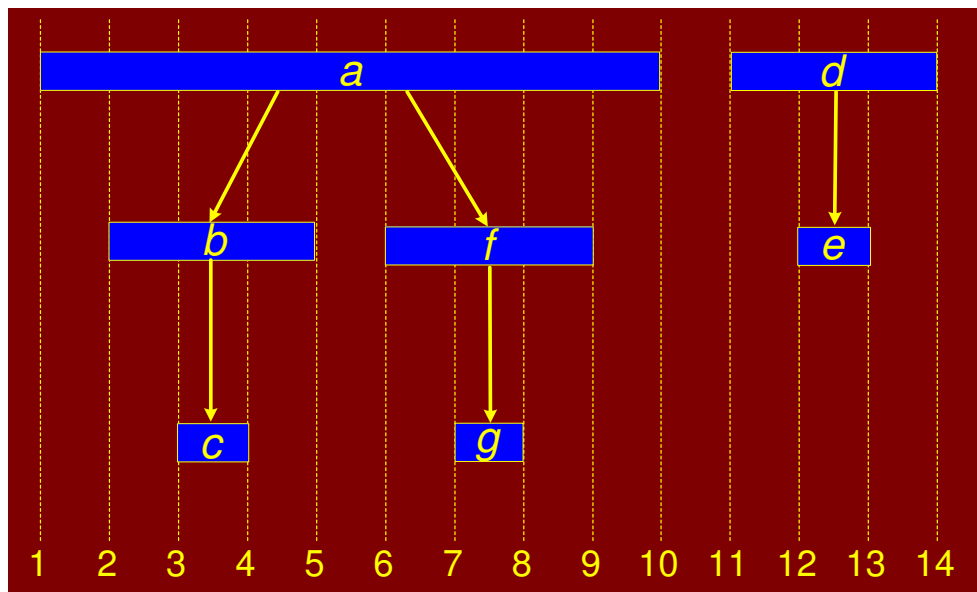
Figure 8.26: Parenthesis lemma
